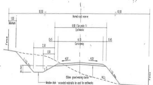
TYPE 6 DISTRICT ROAD (ROLLING TERRAIN)
