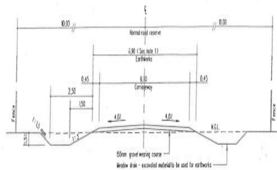
TYPE 6 DISTRICT ROAD (FLAT TERRAIN)
